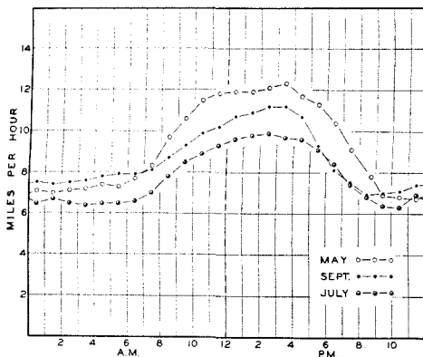
FIG. 5. Average diurnal wind mileage curves for May, July and September at Qu'Appelle, Saskatchewan, computed from hourly records for 1294, 1928, 1932 and 1936.
