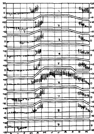
FIG. 4. Soil temperatures ( ^{\circ}\text{C}. ) at Ste. Anne de Bellevue (Macdonald College) during the period Dec. 1930 to Feb. 1939. Solid lines show weekly range at a depth of 4 in., dotted lines the range at 8 in. Summer figures are omitted for all years but 1936. Arrows indicate probable dates at which soil thawed at 4 in.
