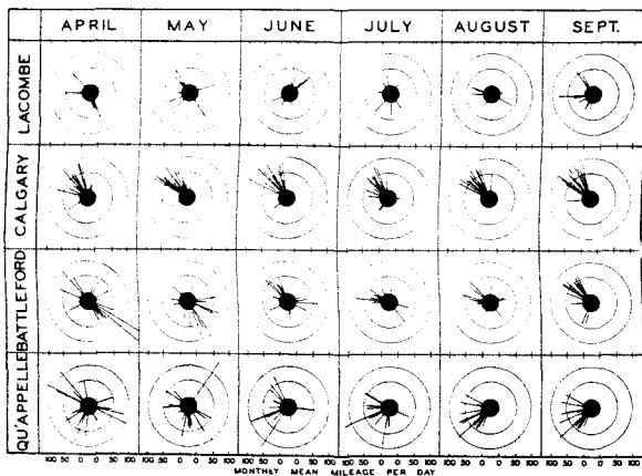
FIG. 2. Resultant wind vectors. Length of vectors indicates mean mileage per day.
