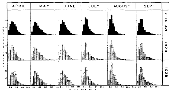
FIG. 6. Percentage frequency distribution of hourly wind mileage at Lacombe, Alberta. Two-year average superimposed upon individual histograms by vertical bars.
