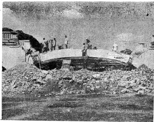
The arch bridge at Kumbakonam being strengthened with concrete keys.
