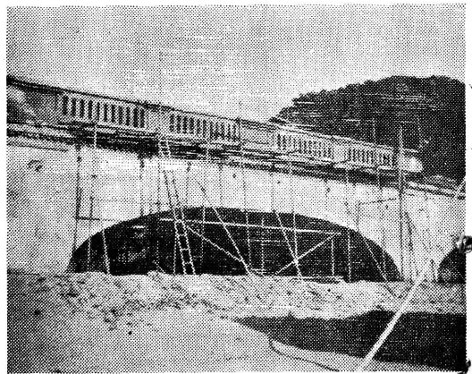
The Bridge after strengthening is ready for test.
