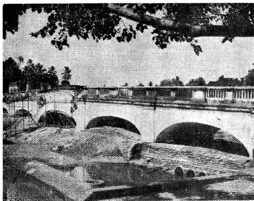
The Kumbakonam arch bridge with scaffolding.
