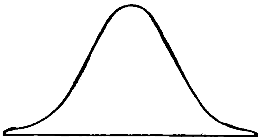
FIG. 1.—The Normal Curve of Distribution.
