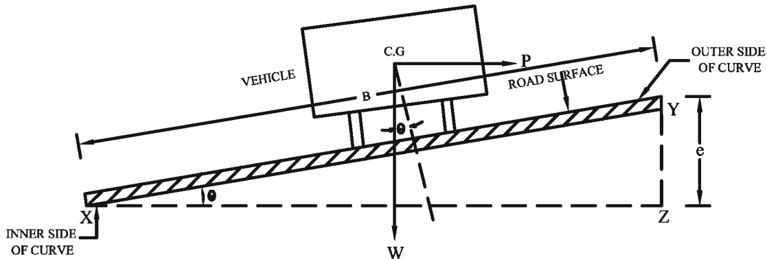
Fig. 8.3 SUPER ELEVATION
