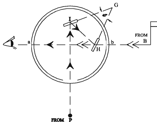
Fig. 6.8 OPTICAL SQUARE
