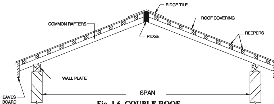
Fig. 1.6. COUPLE ROOF
