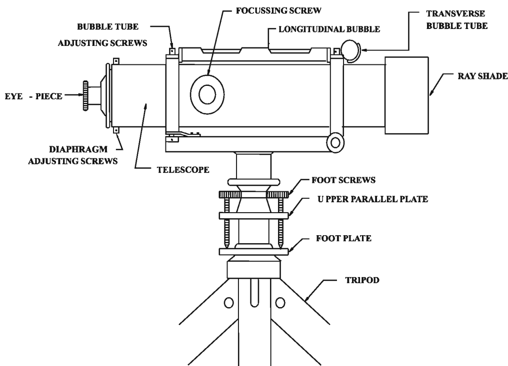
Fig. 6.14 DUMPY LEVEL
