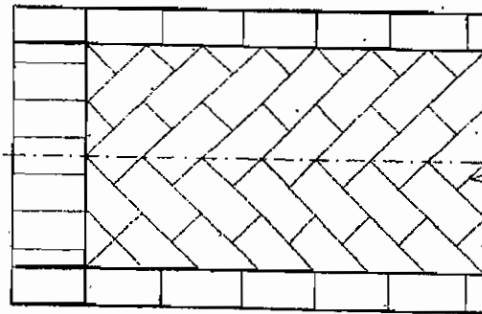
Herring-bone bond
