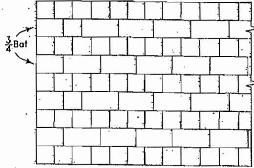
Dutch bond
