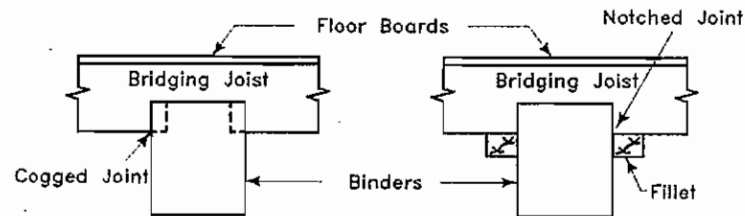
Plan of double joist timber floor
