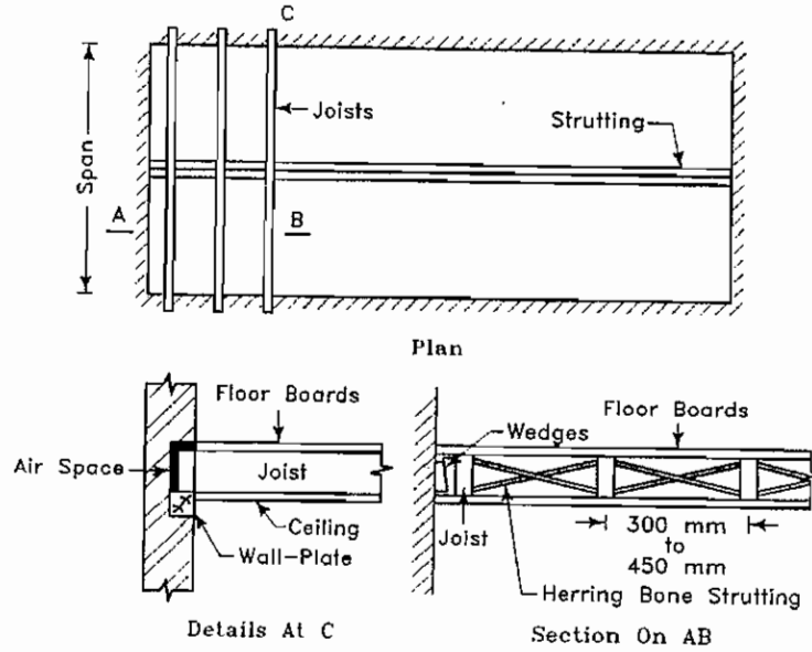
Details of single joist timber floors
