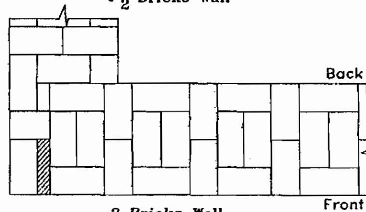
2 Bricks Wall
