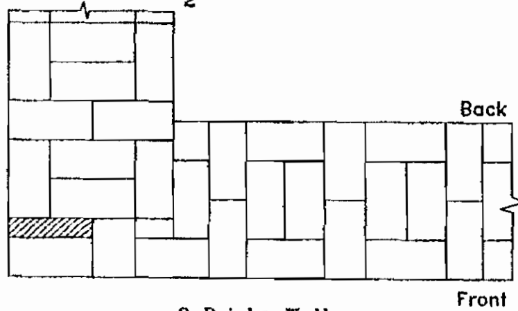
2 Bricks Wall
