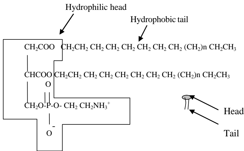
Structure of phospholipid
