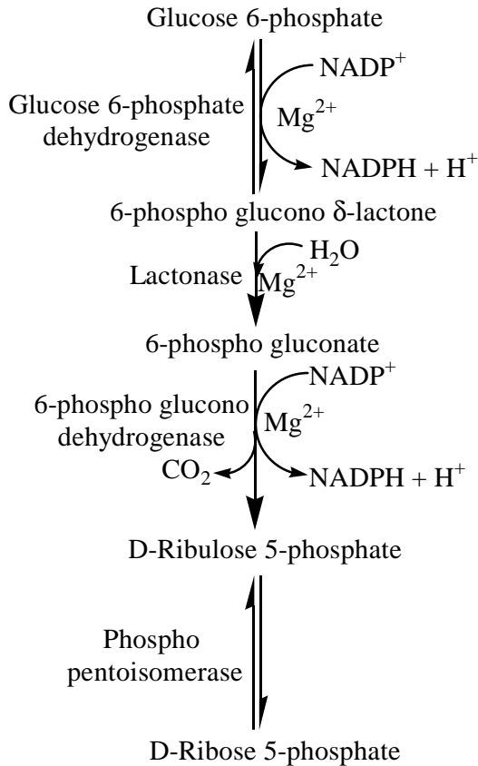
Fig. 3.3 Oxidative reactions of the hexose mono-phosphate pathway
