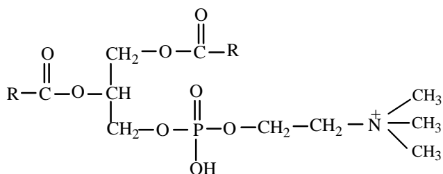
Lecithin
