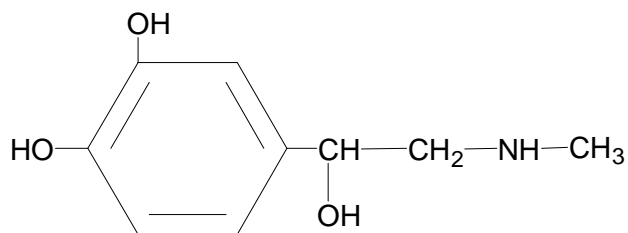
Epinephrine (Adrenaline)
