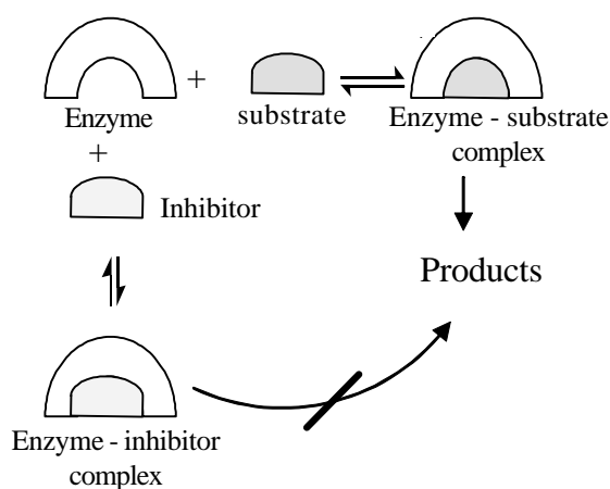
Fig. 9.6 Competitive inhibition
