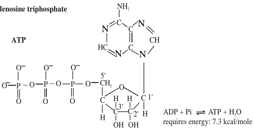
Fig.8.6 Adenosine triphosphate
