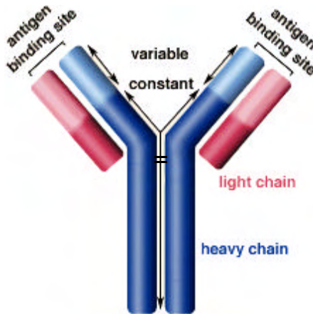
Fig. 10.6 Antibody Structure
