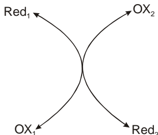
Fig. 8.1 Oxidation-Reduction System
