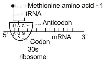
Fig.4.2 Formation of preinitiation complex
