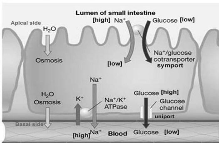
Fig 2.1 Model of glucose absorption
