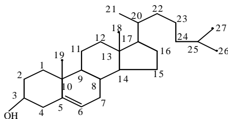
Structure of Cholesterol
