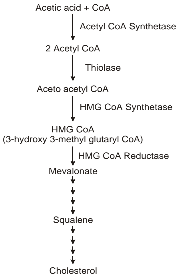
Fig.5.3 Biosynthesis of Cholesterol
