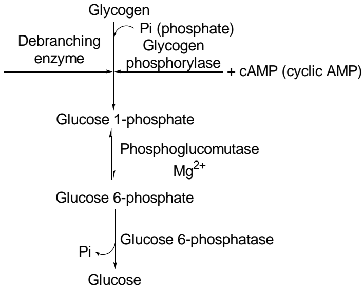
Fig.3.4 Glycogenolysis
