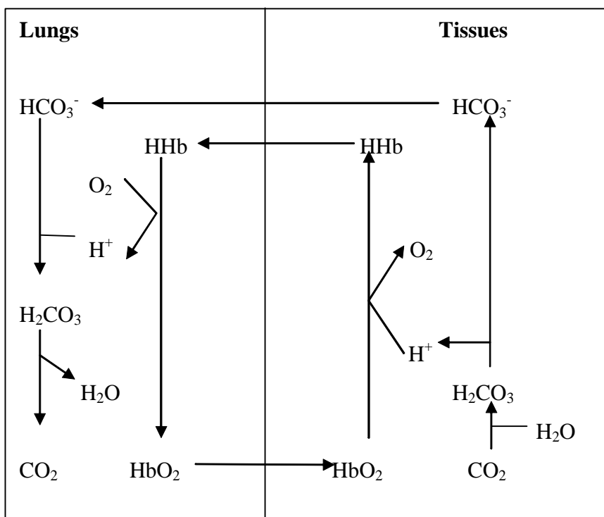
Fig. 1.7 Buffering action of Hemoglobin
