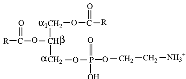
Structure of Cephalin
