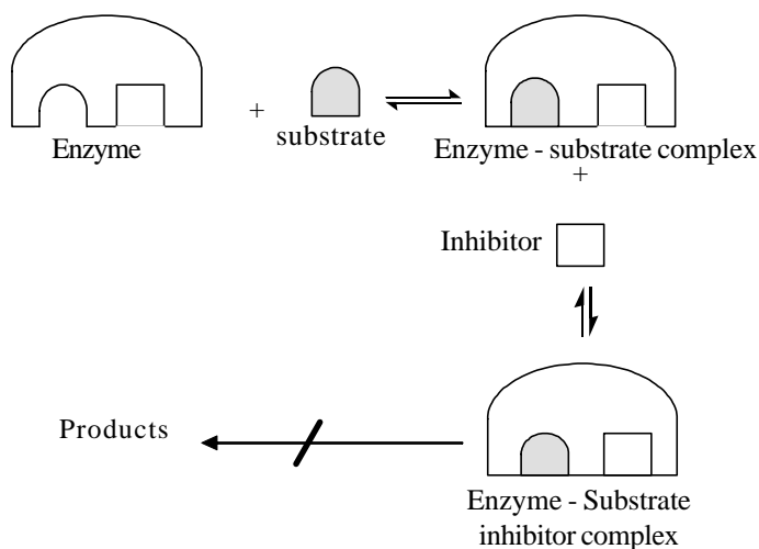
Fig. 9.7 Uncompetitive inhibition
