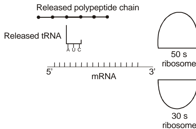
Fig.4.7 Termination of translation
