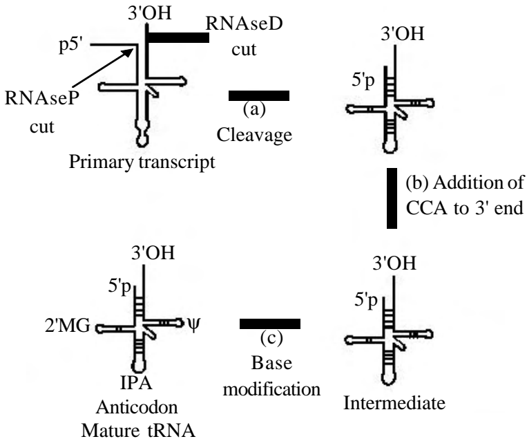
Fig. 6.11 Modification of tRNA molecules
