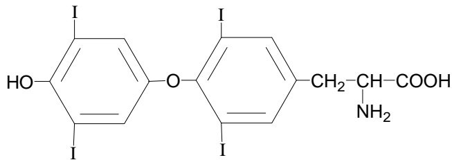
Thyroxine
