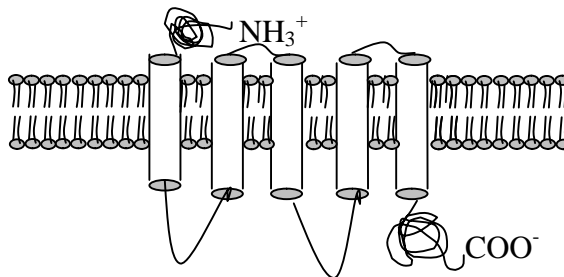
Fig. 1.2 Multipass transmembrane Protein
