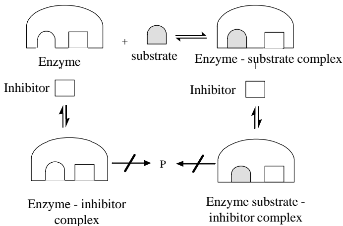
Fig. 9.8 Noncompetitive inhibition
