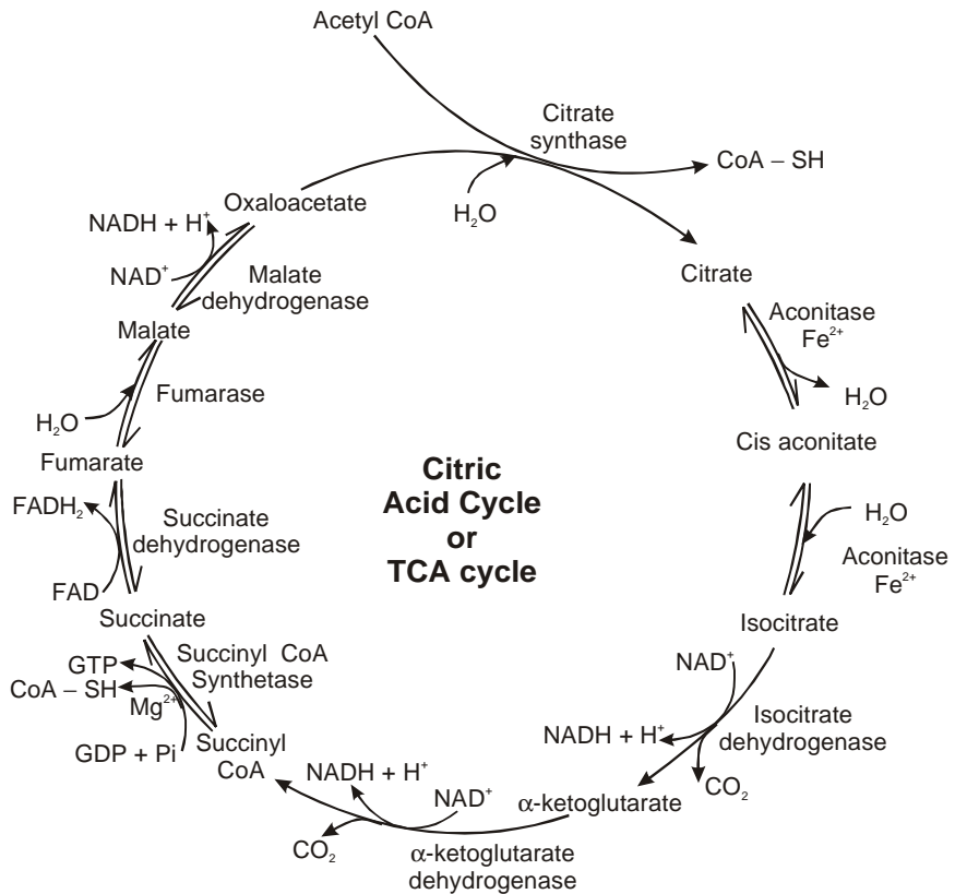
Fig.3.2 Krebs Cycle
