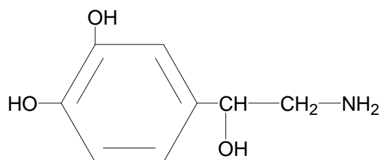
Norepinephrine (Arterenol)
