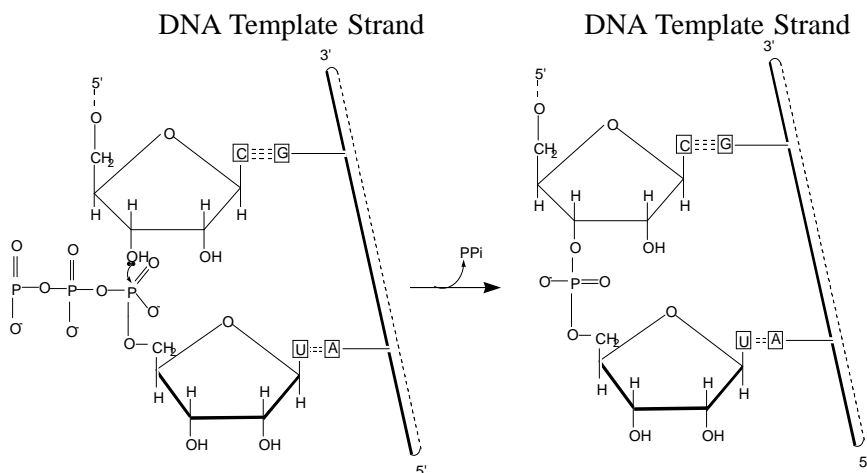
Fig. 6.8 Transcription by RNA polymerase
