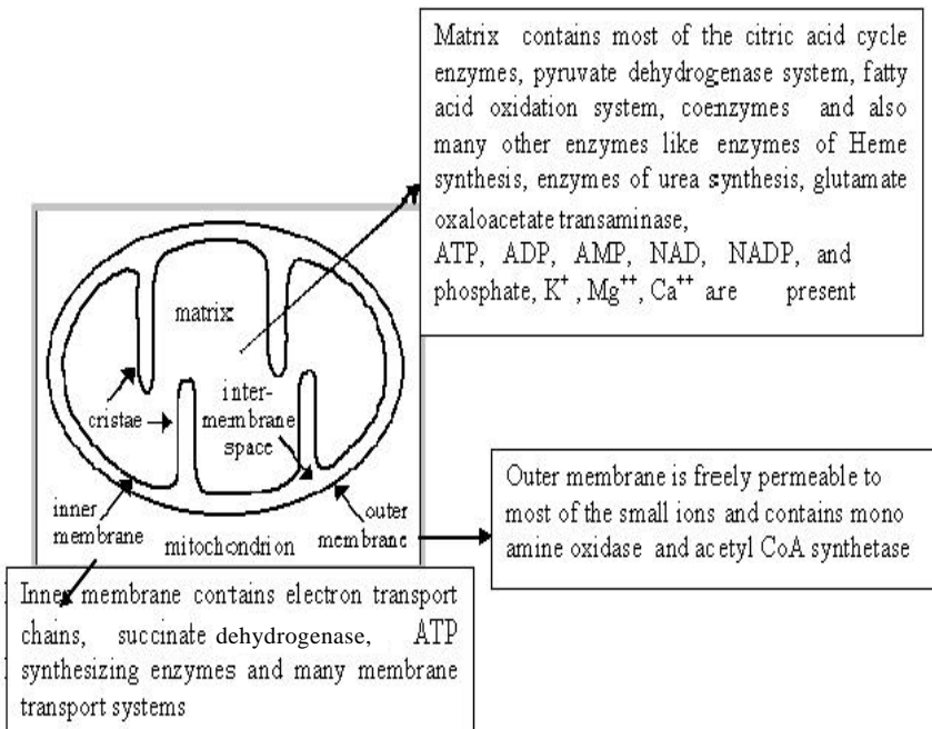
Fig. 8.3 Structure of Mitochondria
