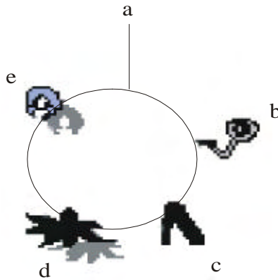
Fig 10.4 Antigen
