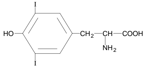
3,5-Diiodotyrosine
