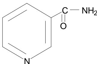
Nicotinamide
