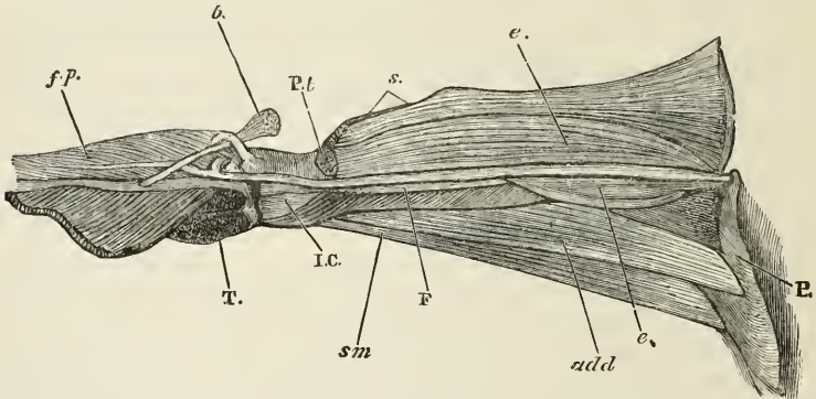
Thigh of Touraco ( Corythoix ) viewed from the inner side, to show the ambiens muscle, arising from the prepubic side of the pelvis ( P ) and running along to blend with one of the tendons of origin of the flexor perfor. digitorum ( f.p. ).— F , femur; Pt , patella; I.C. , inner condyle of femur; T , tibia; b , biceps (cut short); s , sartorius (also cut); e , e , extensor femoris; sm , semimembranosus; add , adductores.
