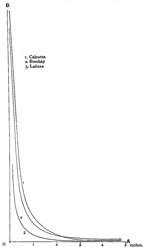
FIG. 31.—CURVES OF RELATIVE RAINFALL FREQUENCY AND QUANTITY.
