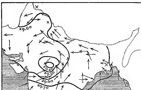
FIG. 22.—WEATHER CHART FOR 10 A.M., 2d July 1883.
