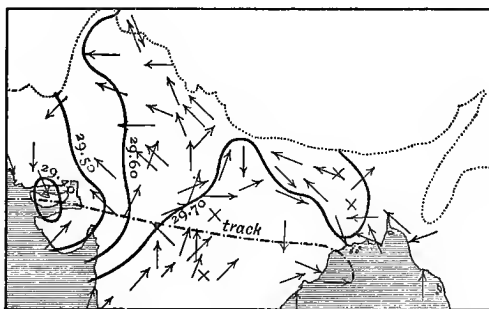
FIG. 23.—WEATHER CHART FOR 10 A.M., 3d July 1883.
