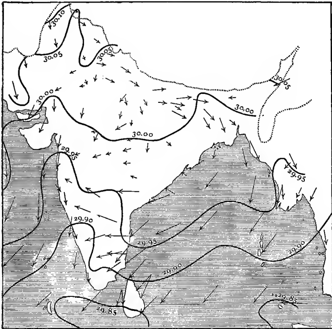
FIG. 3.—AVERAGE BAROMETRIC AND WIND CHART FOR JANUARY.
