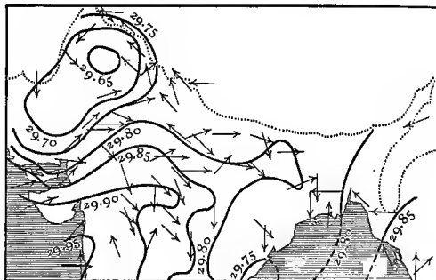
FIG. 19.—WEATHER CHART FOR 10 A.M., 14th September 1882.
