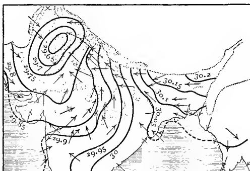
FIG. 13.—WEATHER CHART FOR 10 A.M., 25th January 1883.
