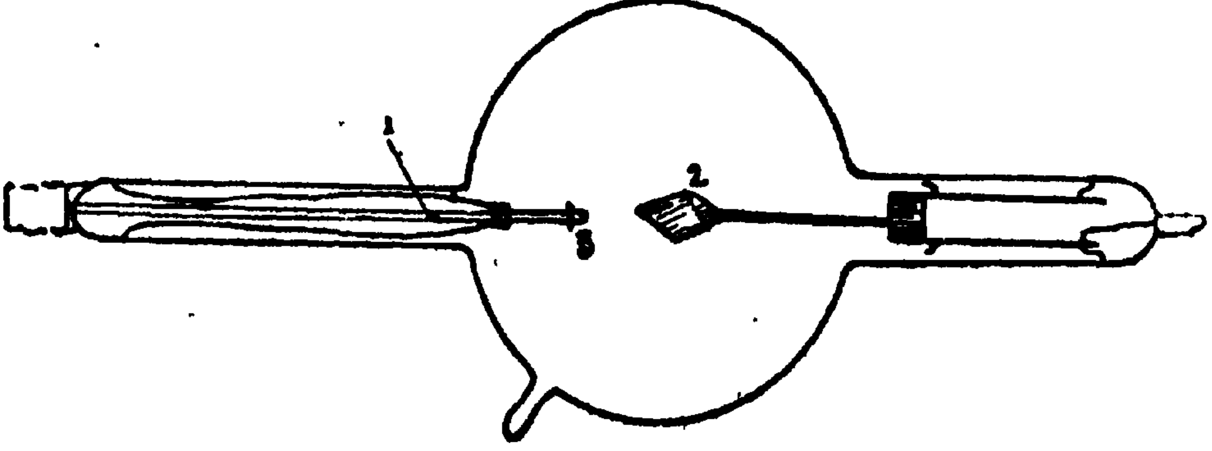
Coolidge X-ray tube.
