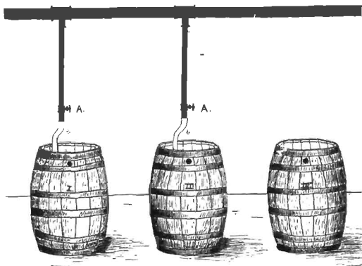
FIGURE 19.—Barrels arranged for the hot-water method of seed treatment. I, tempering bath. II, treating bath. III, cold-water supply. A, shut-off valves. b, rubber hose.
