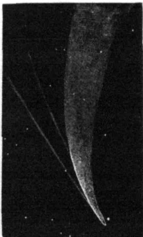
FIG. 101.—Head of Donati's comet of 1858.
