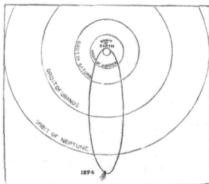
FIG. 99.—Orbit of Halley's comet.
