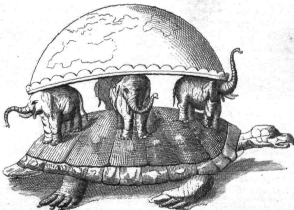
FIG. 6.—Hindoo Earth.
