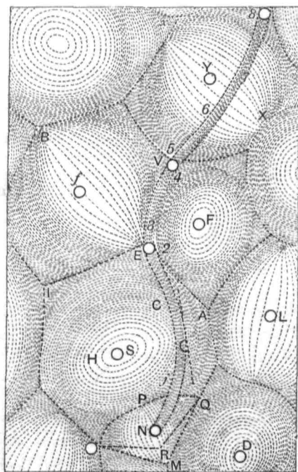
FIG. 55.—Descartes's diagram of vortices, from his Principia .
