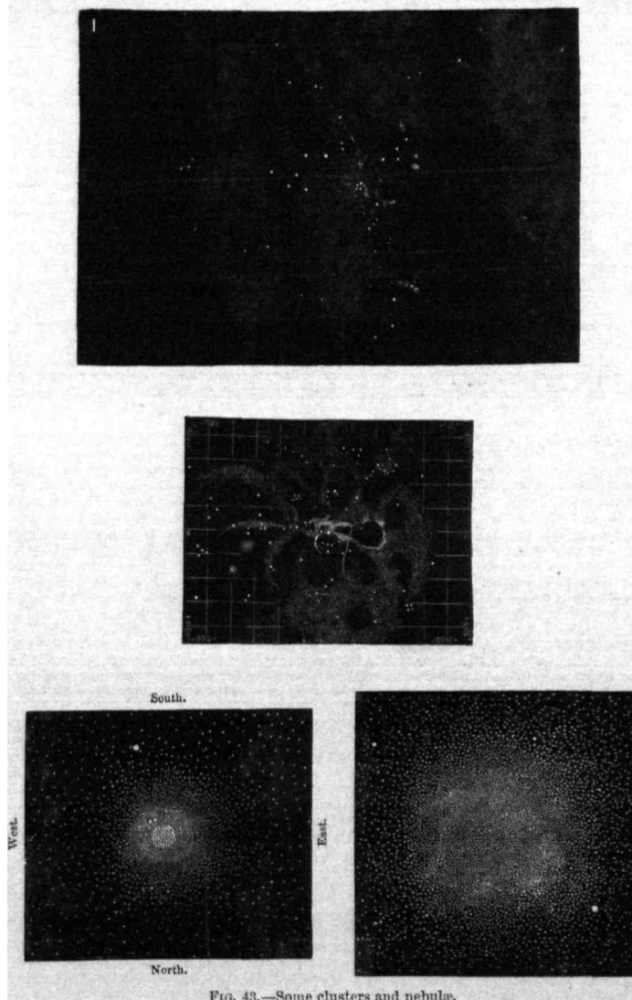
FIG. 43.—Some clusters and nebulae.
