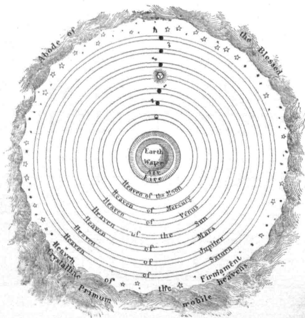
FIG. 8.—Ptolemaic system.
