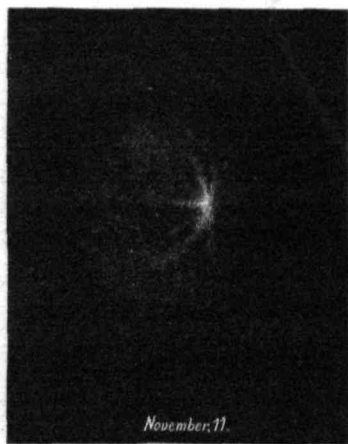
FIG. 103.—Encke's comet.
