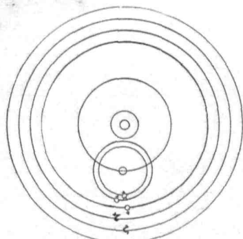
FIG. 11.—Egyptian system.
