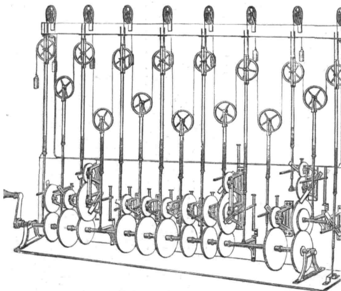
FIG. 119.—Tide-predicter, for combining the ascertained constituents into a tidal curve for the future.
