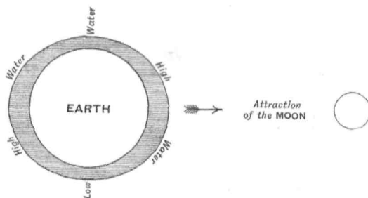
FIG. 112.—Earth and moon (earth's rotation neglected).
