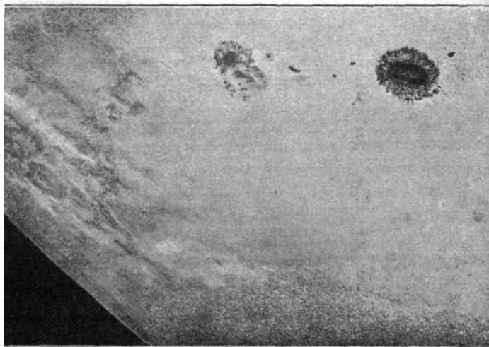
FIG. 49.—A portion of the sun's disk as seen in a powerful modern telescope.
