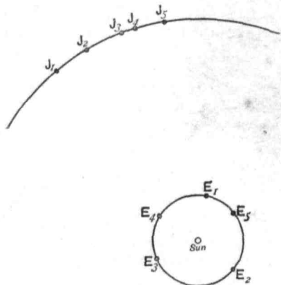
FIG. 12.—True orbits of Earth and Jupiter.
