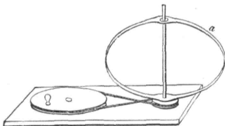
FIG. 110.—Whirling earth model.
