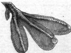
Fig. 126.—Left foot of Podiceps cristatus . 4.
