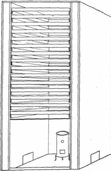
FIG. 4.—Plan of a small stove drier in perspective, with one side removed to show the arrangement of the stove and trays.
