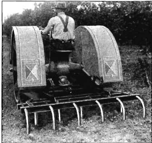
FIG. 138. Spring-tooth harrow and tractor outfit for cultivating
