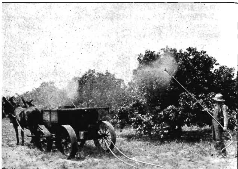
FIG. 221. Power spraying outfit at work in a citrus grove
