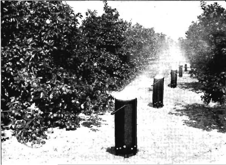
FIG. 159. Coke-heaters in use in a Florida citrus planting
