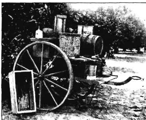
FIG. 226. Cart outfit for handling cyanide, acid and water used in generating gas by the "pot method."
