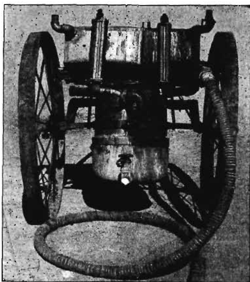
FIG. 227. Machine for generating hydrocyanic-acid gas
