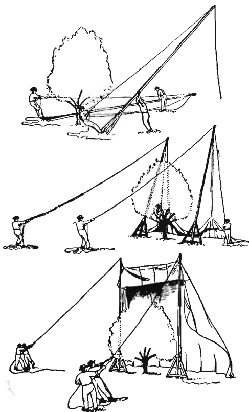
FIG. 230. Covering a large citrus tree with a tent by means of derricks
