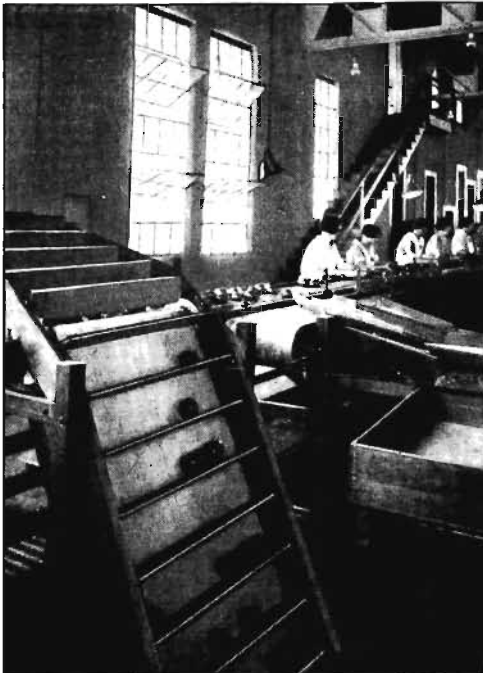
FIG. 177. Grading-belt and graders at work. The elevator which brings fruit from the drier is shown in the foreground
