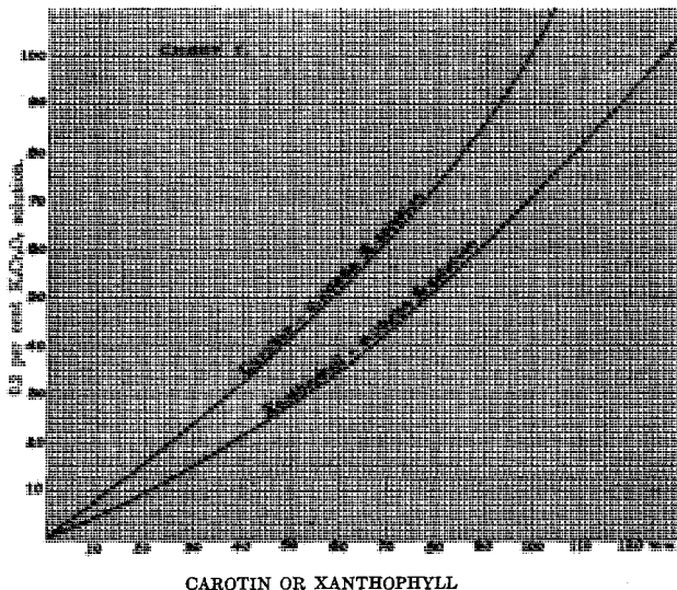
Quantitative relations between 0.2 per cent K_2Cr_2O_7 solutions and 5 \times 10^{-5} molar solutions of carotin and xanthophyll.
