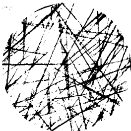
FIG. 5. Lycopin from carbon disulfide-alcohol. ( \times 165 )
