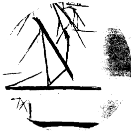
FIG. 6. Fucoxanthin from methyl alcohol.
