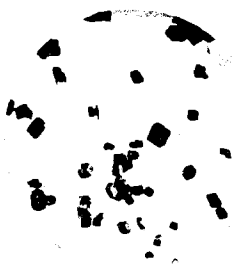
FIG. 1. Carotin from carbon disulfide-alcohol. ( \times 62 )
