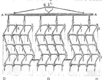
FIG. 18.—ZIZZAG HARROW.
