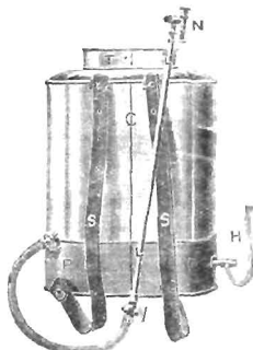
FIG. 262.—KNAPSACK SPRAYING MACHINE.
