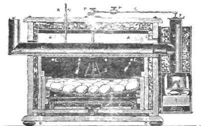
FIG. 235.—TANK INCUBATOR.
