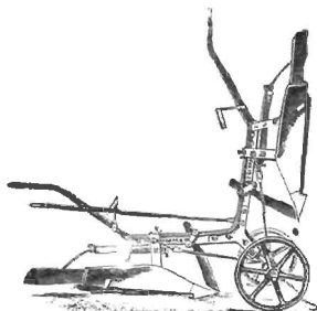
FIG. 14.—TURN-WREST PLOUGH.
