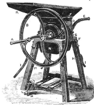
FIG. 37.—TURNIP-CUTTER.
