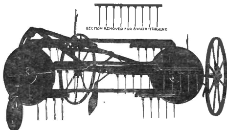
FIG. 25.—COMBINED SIDE RAKE, SWATH TURNER, TEDDER AND WINDROWER.
