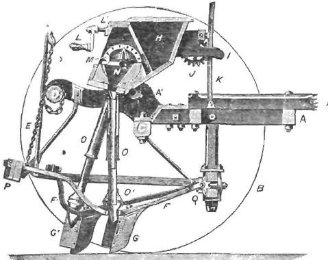
FIG. 20.—CUP DRILL, VERTICAL SECTION (ON LARGER SCALE), SHOWING PARTS.
