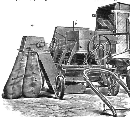
FIG. 36.—STEAM-POWER CHAFF-CUTTER, WITH SIFTING, DUSTING, AND BAGGING APPARATUS.
