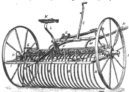
FIG. 26.—SELF-ACTING HORSE-RAKE.
