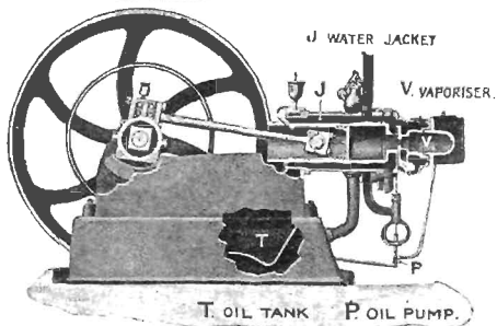
FIG. 32.—OIL ENGINE.
