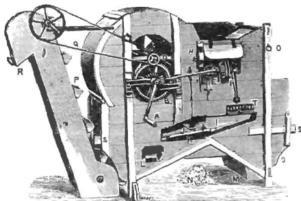
FIG. 33.—CORN WINNOWING OR DRESSING MACHINE.
