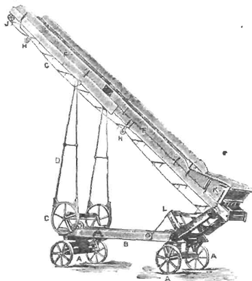
FIG. 27.—STACKING MACHINE OR ELEVATOR.
