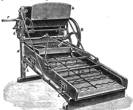
FIG. 34.—ADJUSTABLE FLAT CORN SCREEN.
