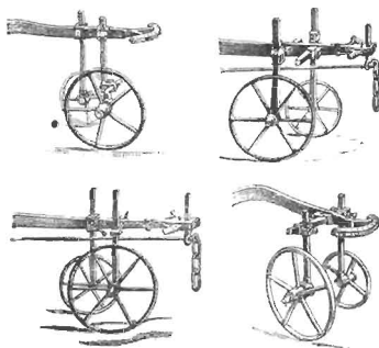
FIG. 8.—PLOUGH WHEELS.
