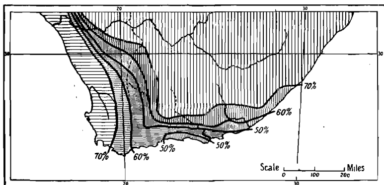
FIG. 25. Proportions of Rainfall in summer (vertical lines) and winter (horizontal lines).
