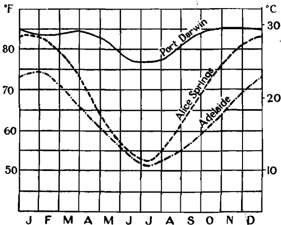
FIG. 139. Curves showing mean monthly temperature. Alice Springs (lat. 24°) is as warm as Darwin (lat. 12°) in summer, but much colder in winter. Adelaide (lat. 35°) has almost the same mean as Alice Springs in winter, but is cooler in summer.
