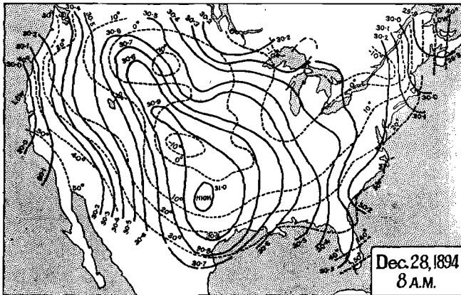
FIG. 102. Pressure and Temperature Conditions during a cold wave in the Mississippi valley and the eastern states. Full lines are isobars, broken lines isotherms, ^{\circ}\text{F} .
