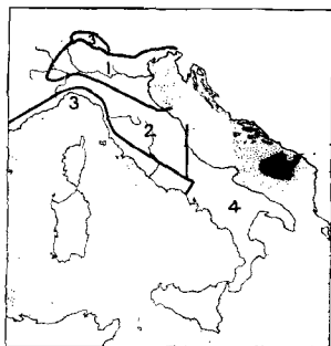
FIG. 96. Major climate regions of Italy.
