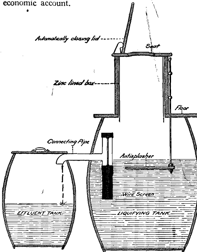
Fig. 40.—The Lumsden, Roberts and Stiles apparatus for the safe disposal of night-soil. (Redrawn from Lumsden, Roberts and Stiles.)
