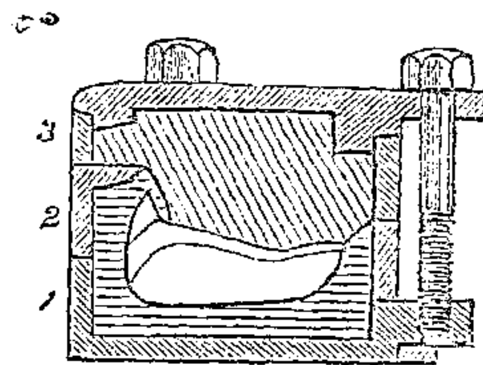
Fig. 66. Three-part Flask in section.
