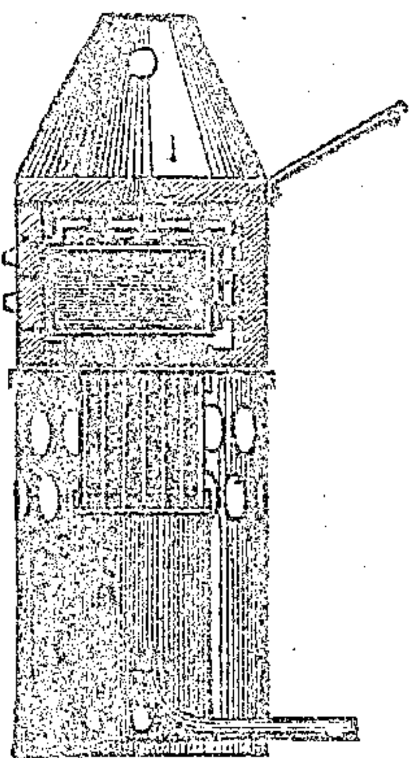
Fig. 82. Muffle Furnace (gas), Fletcher's.
