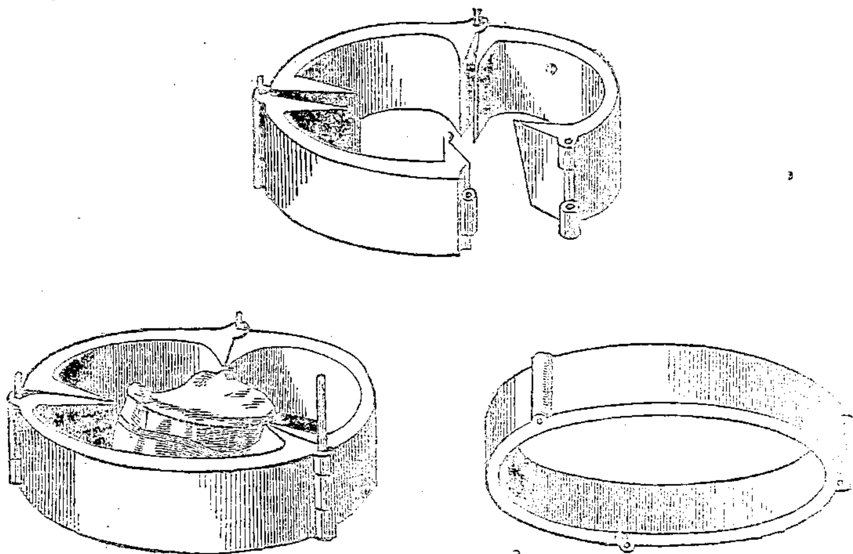
Figs. 15, 16, and 17. Dr. Hayes's Casting Flask.
