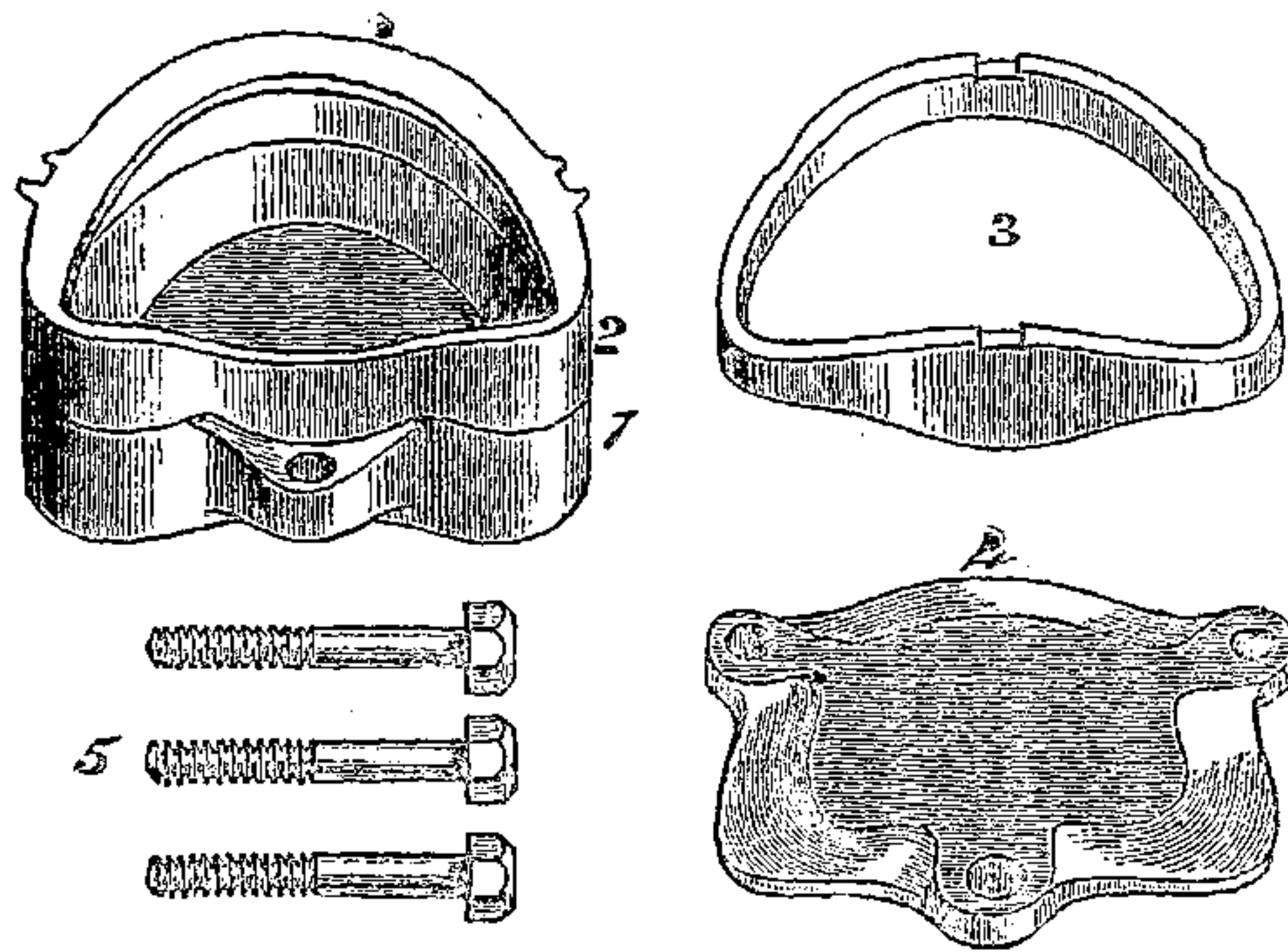
Fig. 65. Three-part Flask.
