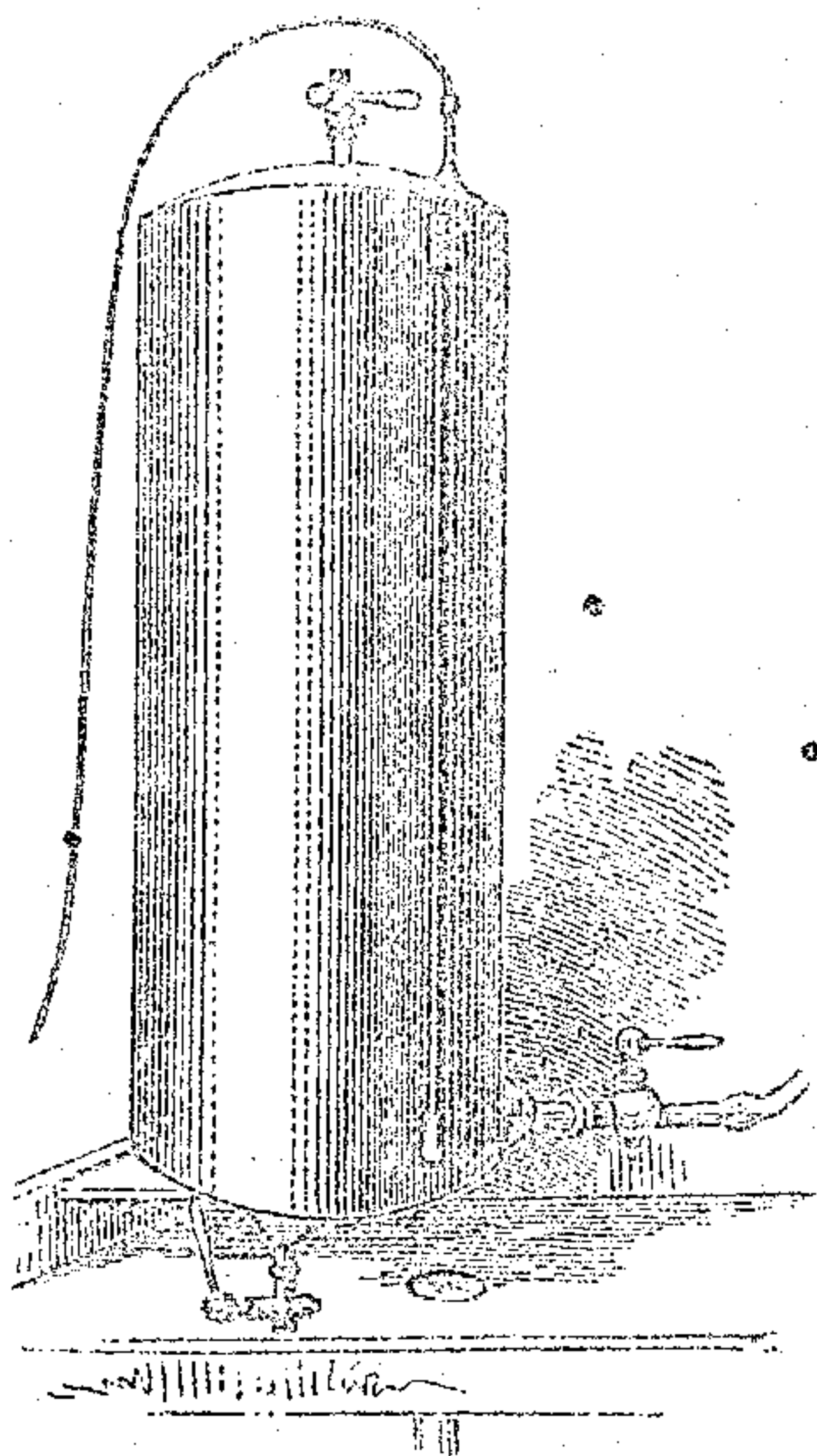
Fig. 29. Hydrostatic Machine for Blowpipe (Richardson's).
