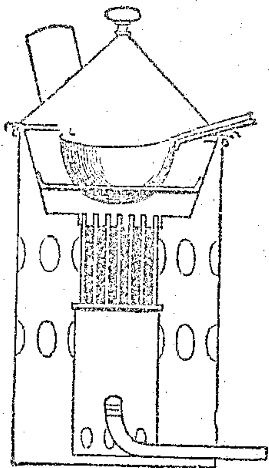
Fig. 18, Fletcher's Stove for Zinc and Lead melting.
