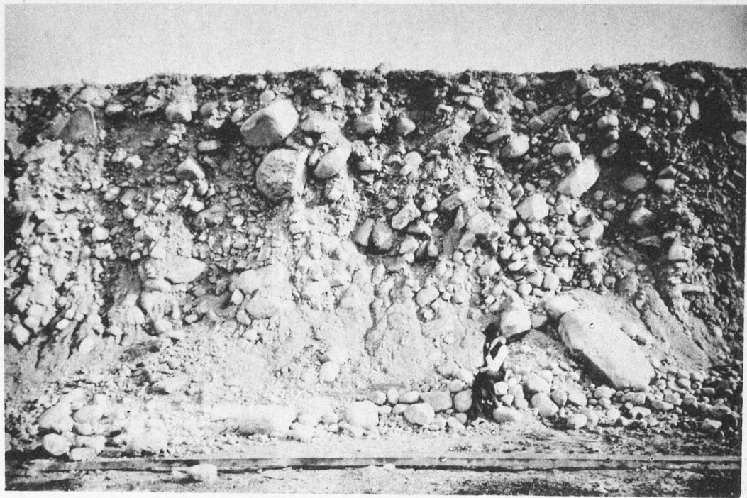
PLATE II. GRAVEL. Chicago Drainage Canal. Photo by O. C. Farrington.
