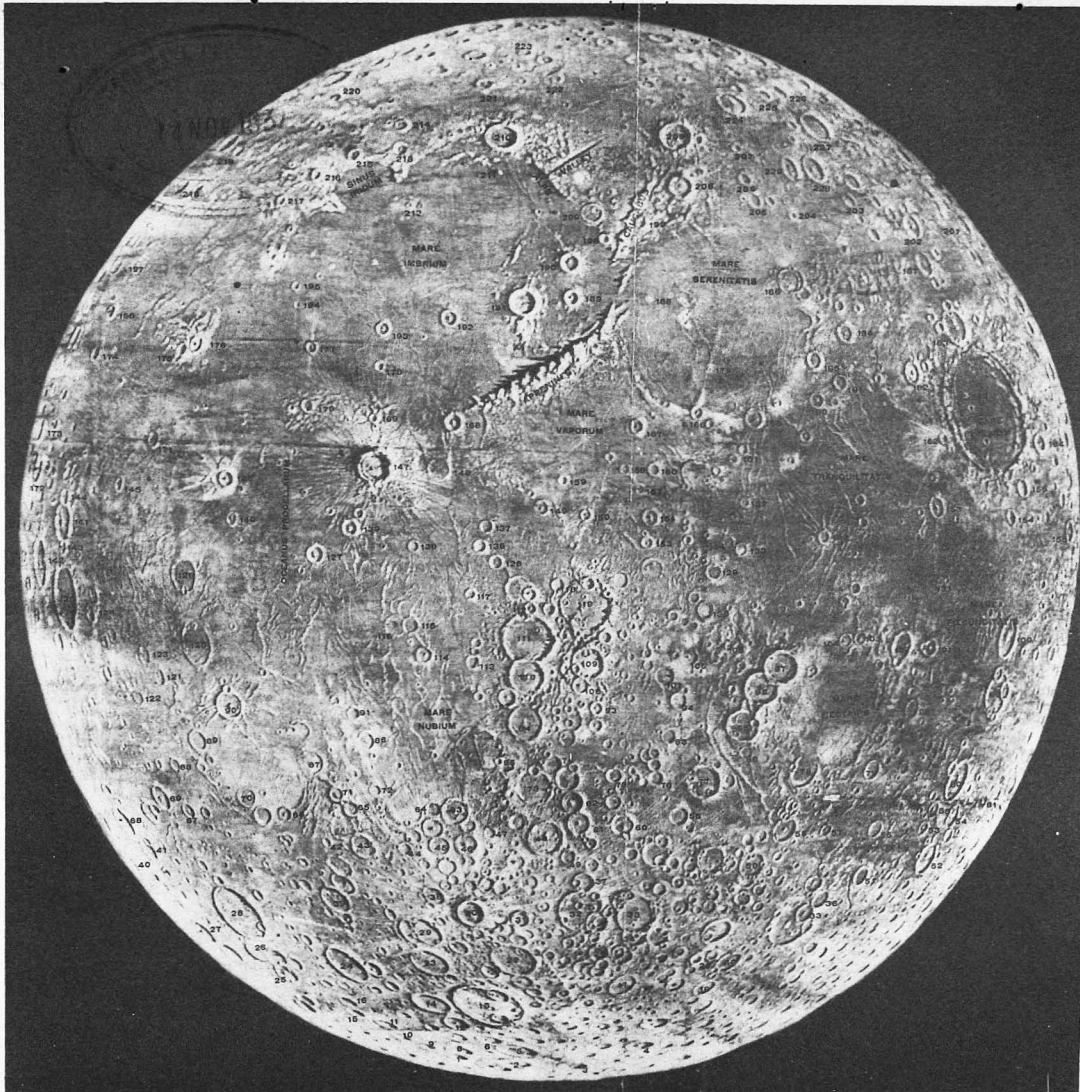
CHART OF THE MOON'S SURFACE. AFTER NASMYTH.
