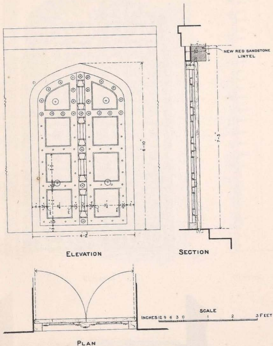
MUGHAL DOOR IN DELHI FORT (See para. 103).
