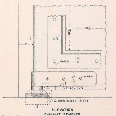
MUGHAL PATTERN DOOR AND ITS FITTINGS (See para. 103).
