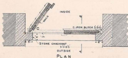
MUGHAL PATTERN DOOR AND ITS FITTINGS (See para. 103).
