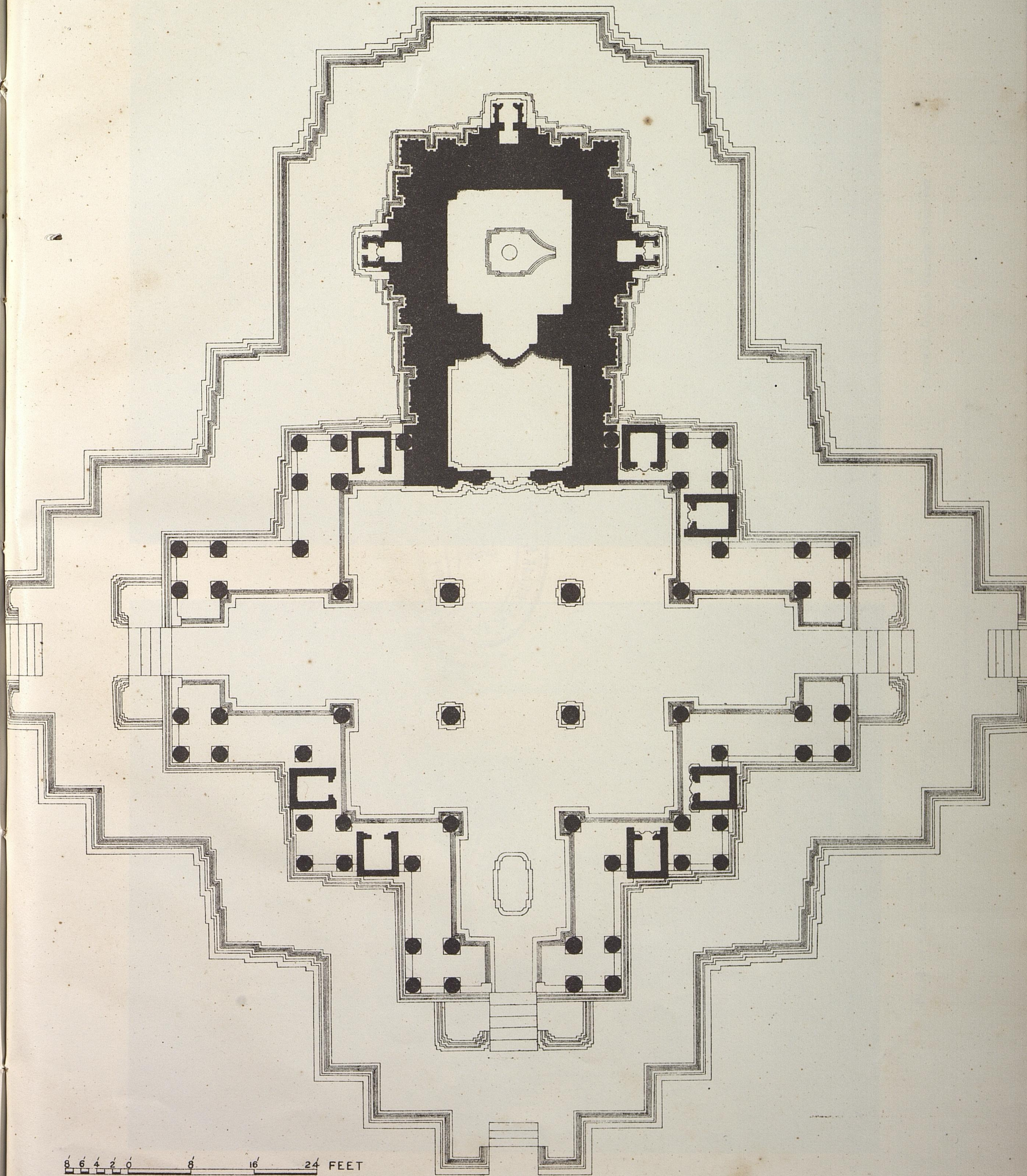
PLAN OF GREAT TEMPLE, PALAMPET.
