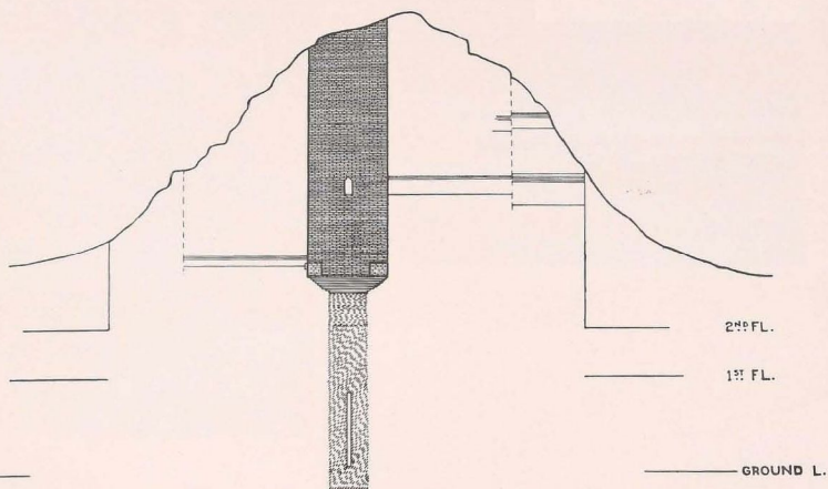
(a) Main Mound. Section of the Central Chamber.
