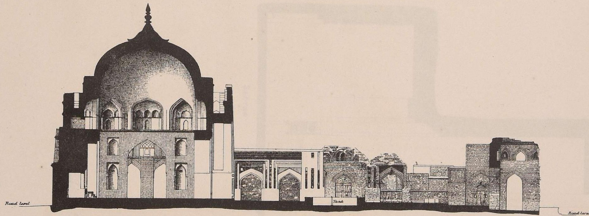
Section through grand dome and east gate.
