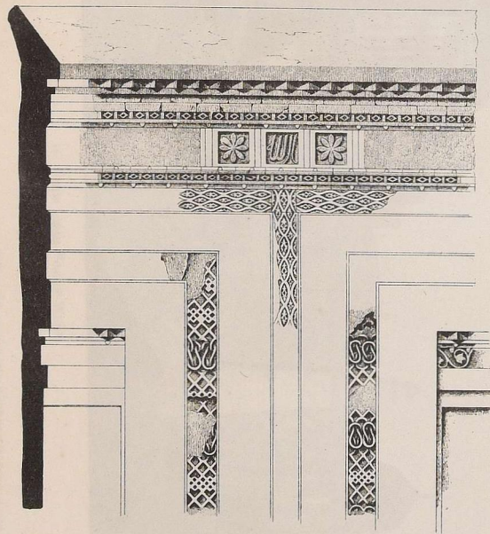
Detail of carved brickwork in cloister arches on south side of courtyard.
