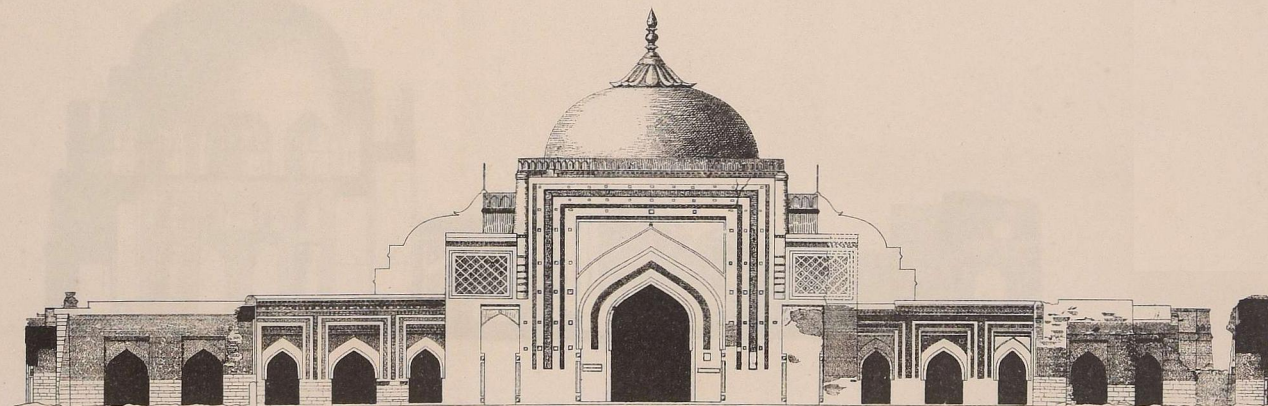
Elevation of west interior façade.
