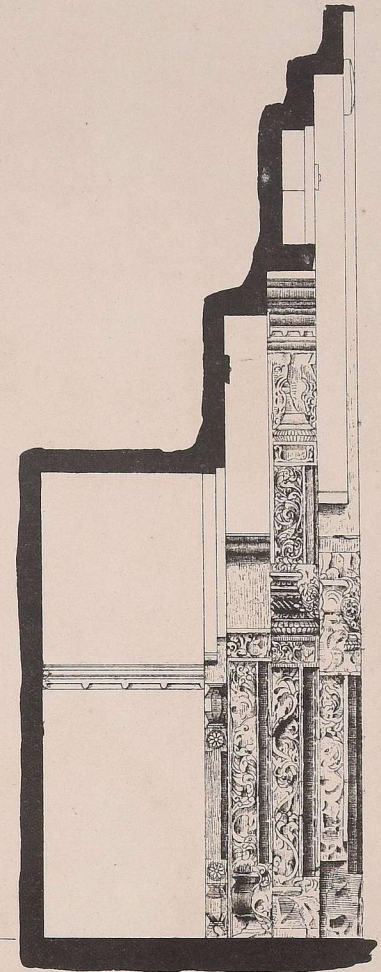
Section
