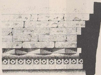
Detail of upper string course at the north angle of the eastern external façade.
