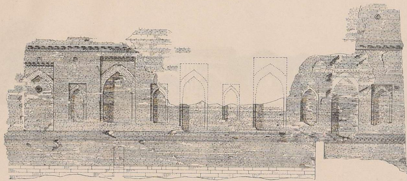
Detail of north angle, east exterior elevation.
