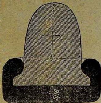
Sectional-view Special-wheel.
