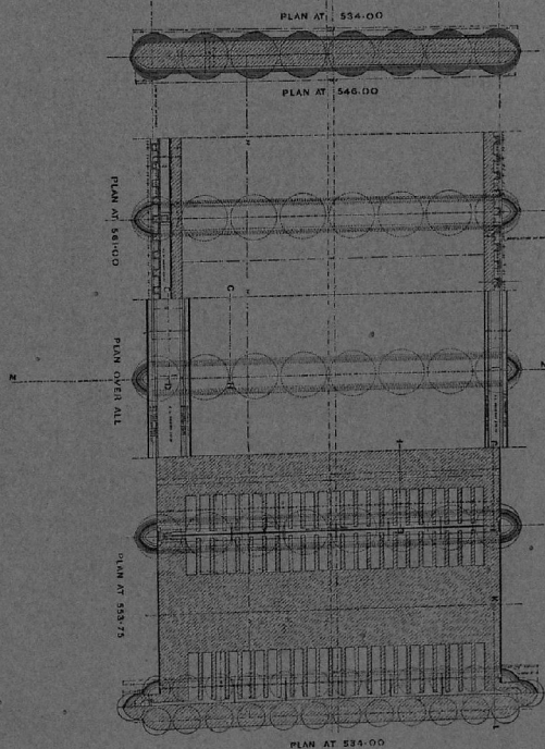
KALI NADI AQUEDUCT ON THE LOWER GANGES CANAL.
