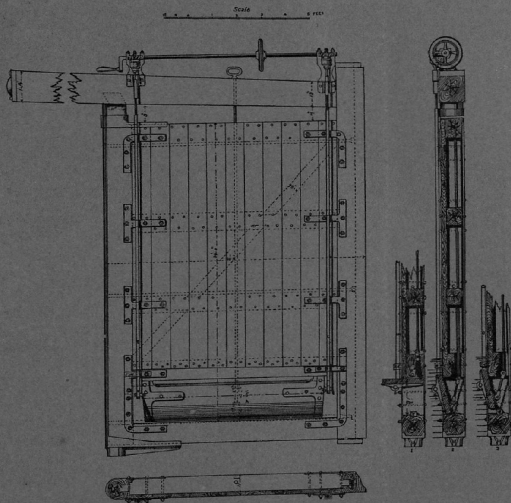
"ER-DUM" VALVE ON ORISSA LOCK GATES.
