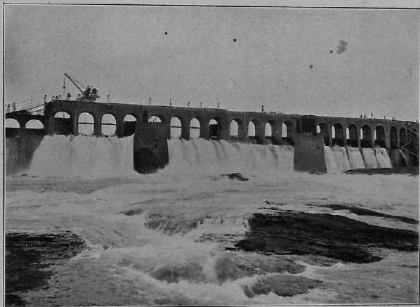
GROUPED AUTOMATIC WASTE-WEIR GATES, LAKE FIFE, BOMBAY.
