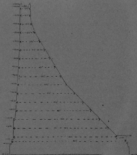
GROSS SECTION OF THE PERIYAR DAM.
