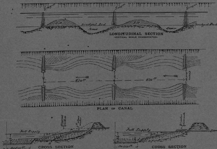
GROYNES ON THE IBRAHIMIAH CANAL.
