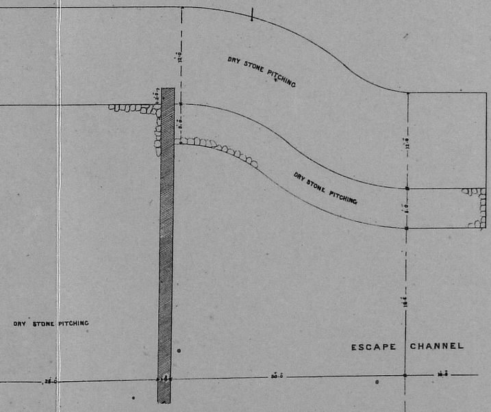
OUTFALL RAPID AT TAIL OF ESCAPE CHANNEL
