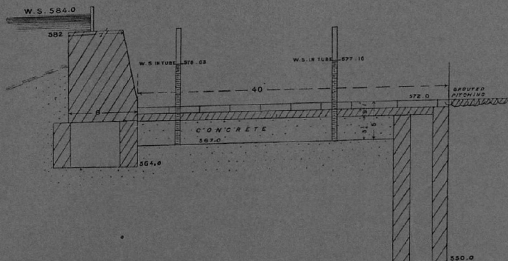
PRESSURE EXPERIMENTS AT NARORA WEIR.
