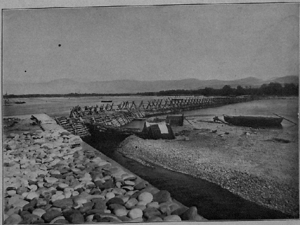
HEAD BUNDS ON THE GANGES CANAL, LOOKING UP-STREAM.
