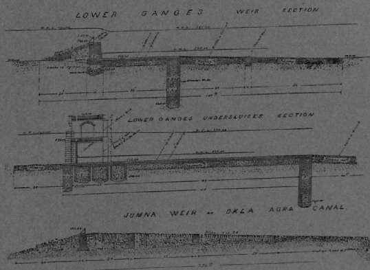
SECTIONS OF THE NARORA WEIR ON THE GANGES AND THE OKLA WEIR ON THE JUMNA RIVER.
