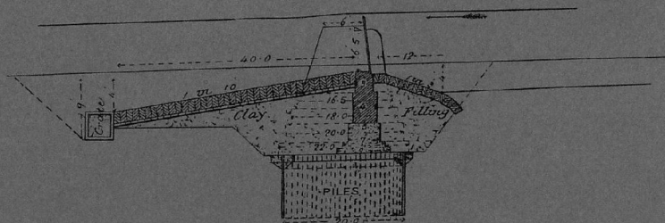
SECTIONS OF SIDHNAI WEIR ON THE RAVI RIVER.
