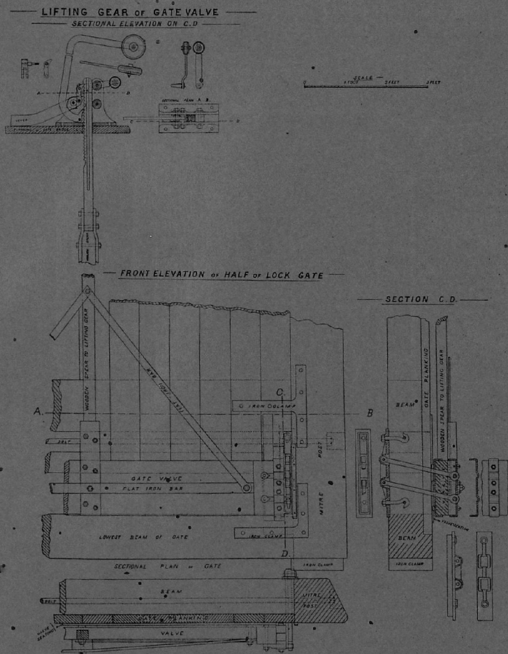
LOCK GATE VALVE ON THE SONE CANALS.
