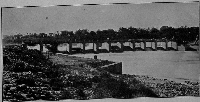
UNDER-SLUICES, MADHOPUR WEIR, BARI DOAB CANAL, DOWN-STREAM.
