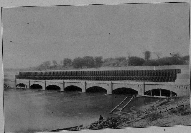
SISWAN SUPER-PASSAGE ON THE SIRHIND CANAL.
