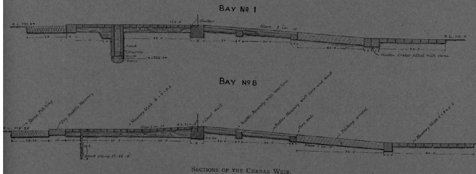
SECTIONS OF THE CHENAB WEIR.
