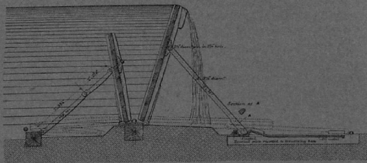
UNDER-SLUICE SHUTTERS USED ON THE ORISSA AND MIDNAPORE CANALS.
