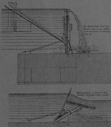
FOURACRES' DOUBLE TUMBLER SHUTTER.
