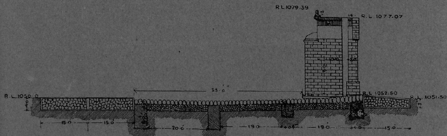
SECTION OF UNDER-SLUICES, WESTERN JUMNA CANAL.
