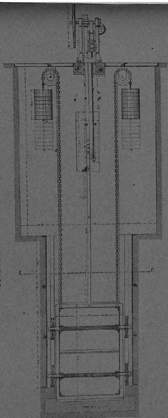
SECTIONAL ELEVATION THROUGH A.B.
