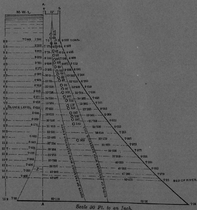
PROFILE OF MARIKANAVE DAM. SPECIFIC GRAVITY, 2.4.
