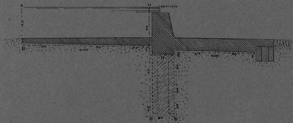
SECTION OF WEIR, SHOWING PATH OF PERCOLATION.
