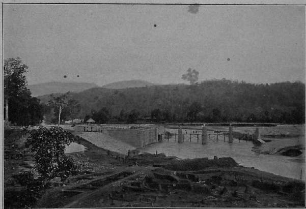
HEAD REGULATOR AND UNDER-SLUCICES OF THE MANDALAY CANAL.
