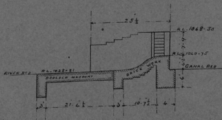
SECTION OF WEIR AT NAUSHERA, EASTERN JUMNA CANAL.
