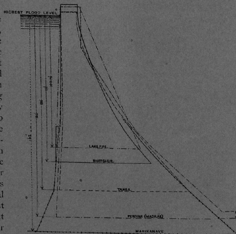
CROSS SECTIONS OF INDIAN MASONRY DAMS.
