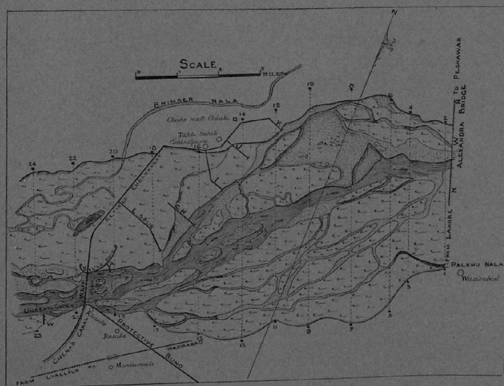
HEAD WORKS OF THE CHENAB CANAL.
