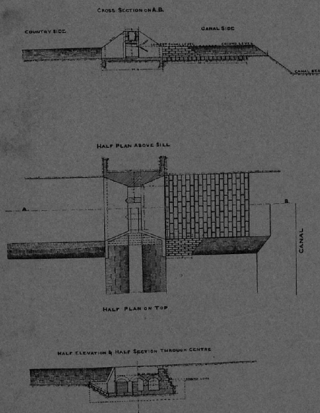
INLET, OUTLET, AND SUPPLY SLUICES ON THE ORISSA COAST CANAL.
