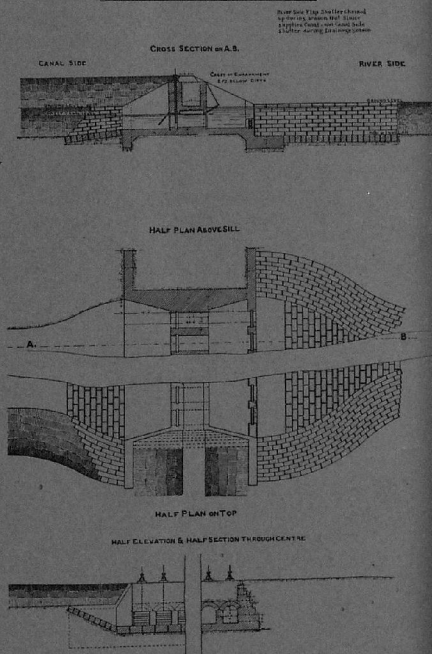
INLET, OUTLET, AND SUPPLY SLUICES ON THE ORISSA COAST CANAL.
