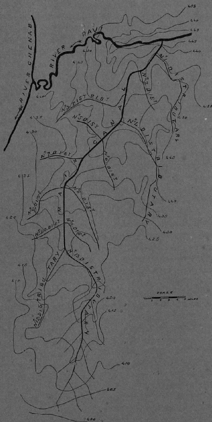
CONTOUR PLAN, SIDHNAI CANAL.
