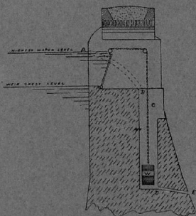
WHITING'S SELF-ACTING WASTE WEIR GATE.
