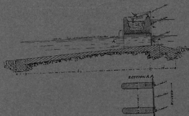
SECTION OF HEAD-SLUICE, BARI DOAB CANAL.
