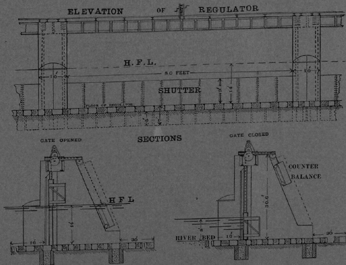
PROPOSED REGULATOR GATES, PENNER RIVER, MADRAS.
