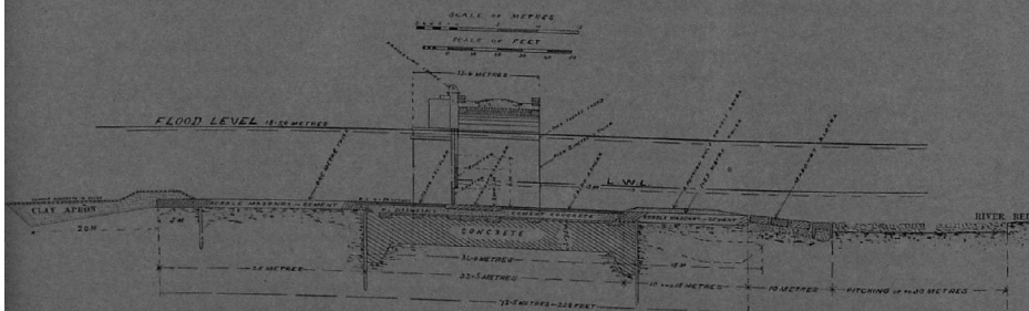
DELTA BARRAGE AS RECONSTRUCTED.
