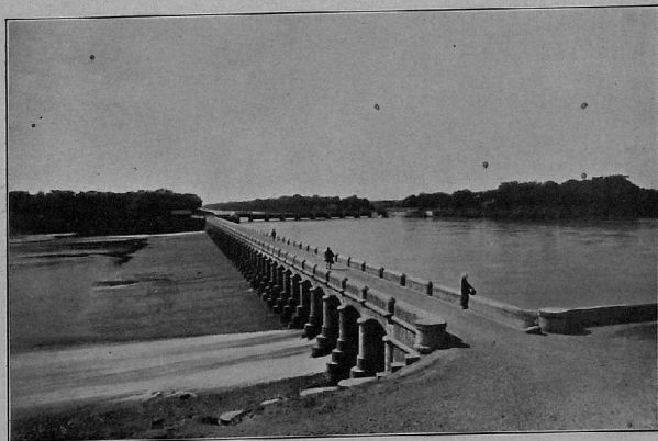
LEVEL CROSSING AT DHANAURI ON THE GANGES CANAL.
