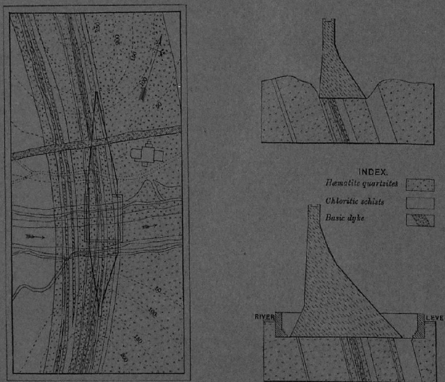
MARIKANAVE DAM, PLAN AND SECTIONS SHOWING FOUNDATIONS.
