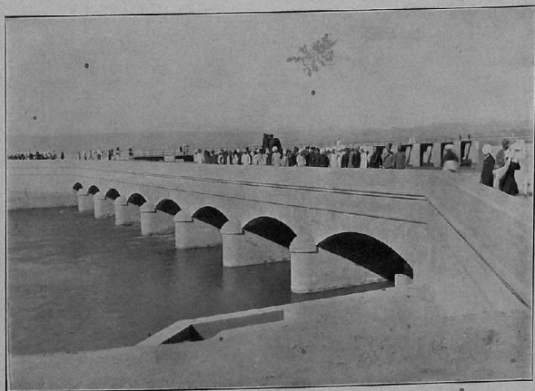
HEAD REGULATOR OF THE JHELUM CANAL.
