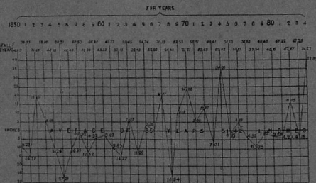
DIAGRAM OF MONSOON RAINFALL AT JUBBULPORE.
