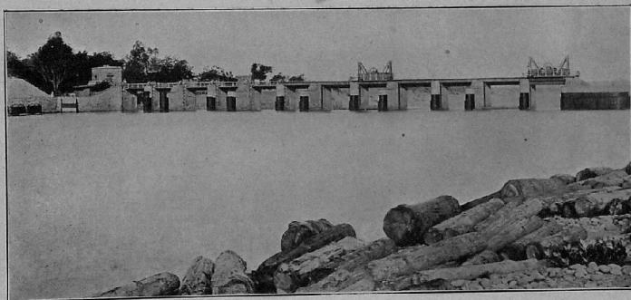
UNDER-SLUICES, MADHOPUR WEIR, BARI DOAB CANAL, UP-STREAM.
