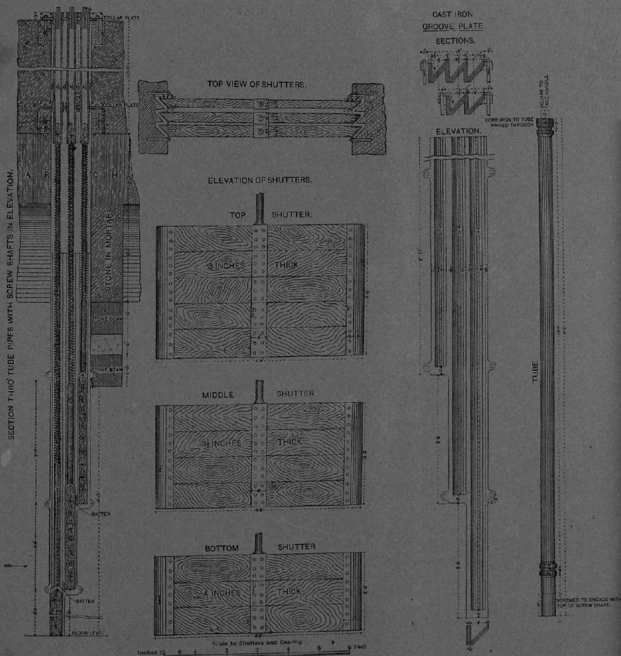
SHUTTERS OF THE BEZWADA HEAD-SLUICE, KISTNA CANALS.
