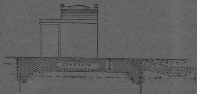
ORIGINAL SECTION OF THE DELTA BARRAGE.
