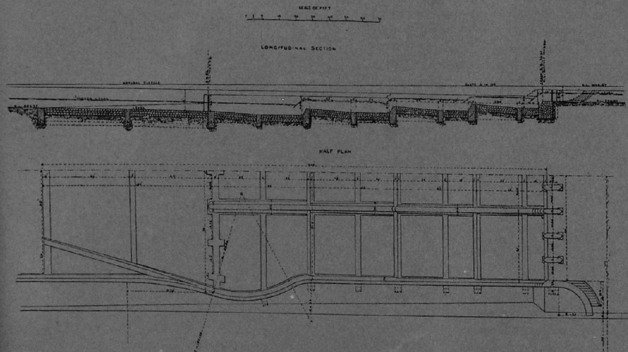
CASCADE FALL ON THE BARI DOAB CANAL.
