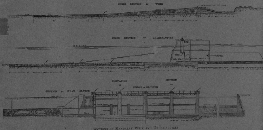
SECTIONS OF MANDALAY WEIR AND UNDERSLUCICES
