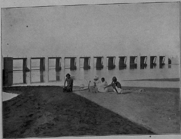
UNDER-SLUICES OF THE JHELM WEIR.
