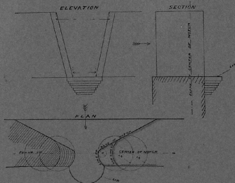
FORM OF NOTCH USED ON FALLS IN THE PUNJAB.
