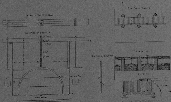
ESCAPE, OR SURPLUS SLUICE, IN MADRAS.
