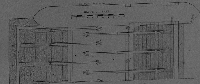
UNDER-SLUICE SHUTTERS OF THE SONE WEIR
