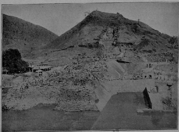
MARIKANAVE DAM UNDER CONSTRUCTION IN 1900.
