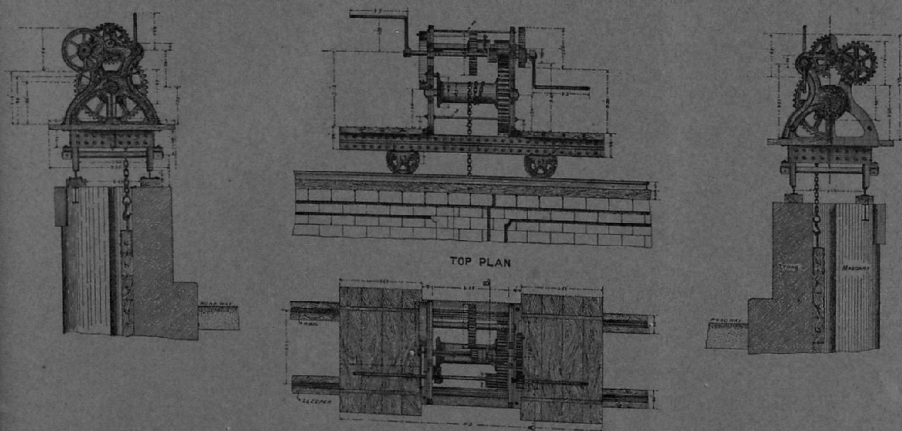
TRAVELLER ON THE HEAD REGULATOR, CHENAB CANAL.
