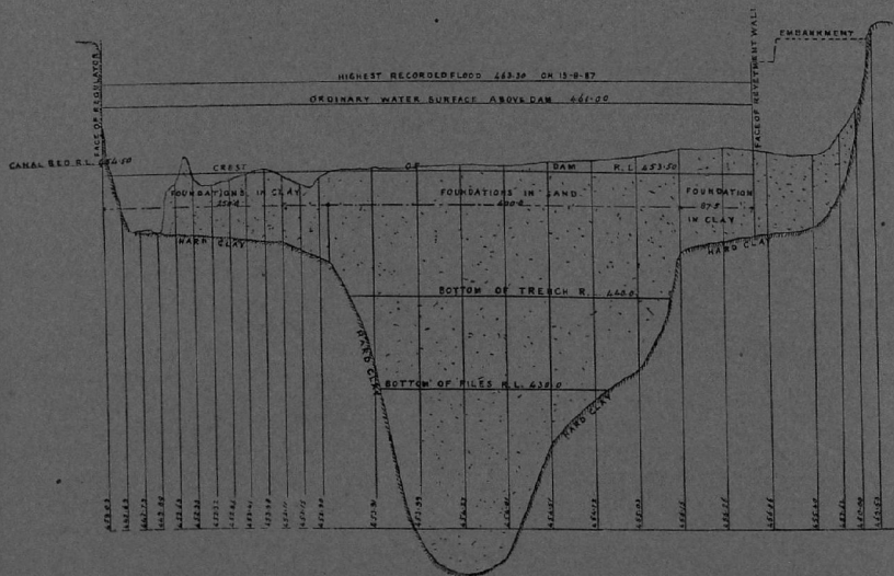
SECTION OF RAVI RIVER AT SITE OF SIDHNAI WEIR.
