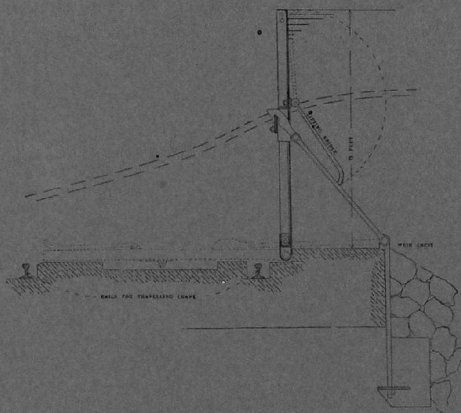
CREST SHUTTERS ON THE ROPAR WEIR, SIRHIND CANAL.
