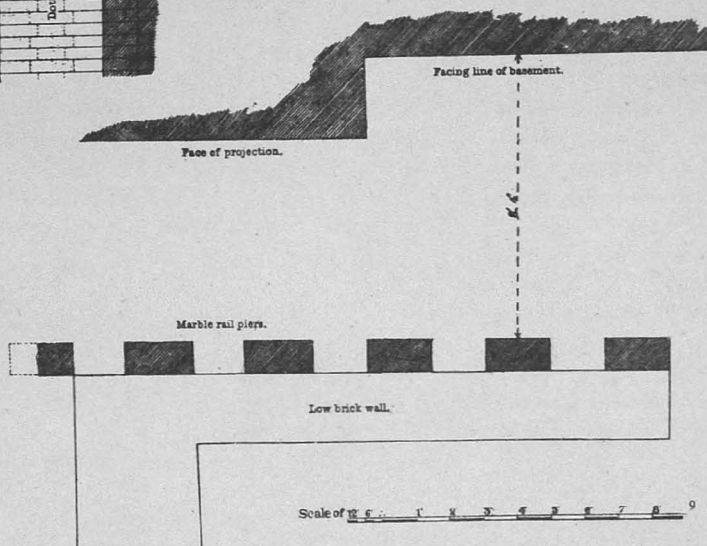
Fig. 5. Plan of Rail Piers, uncovered on north side.
