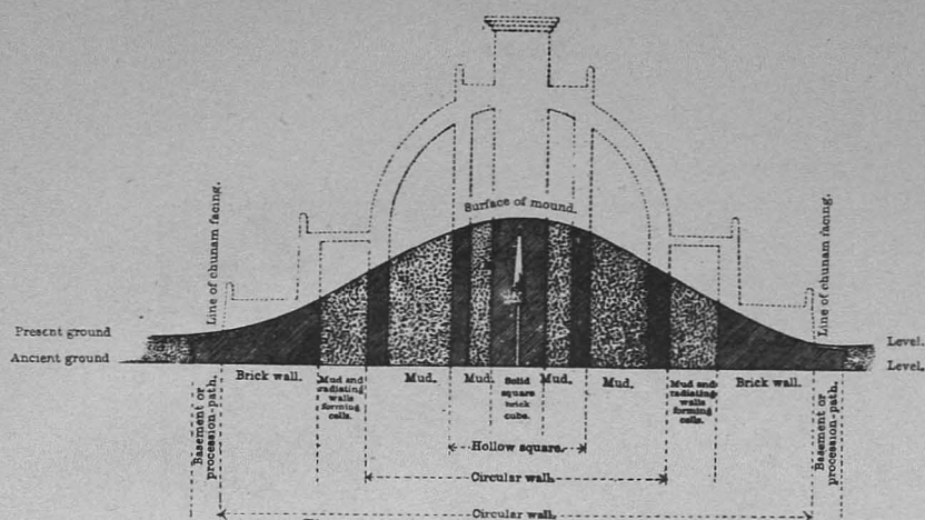
Fig. 1. Section. Dotted lines indicate assumed outline of building.
