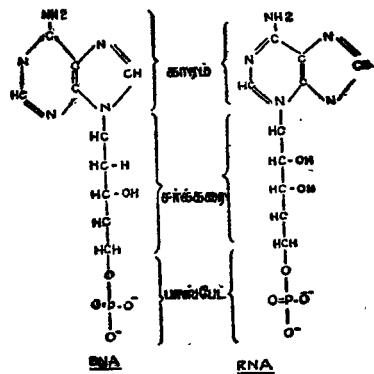
RNA
