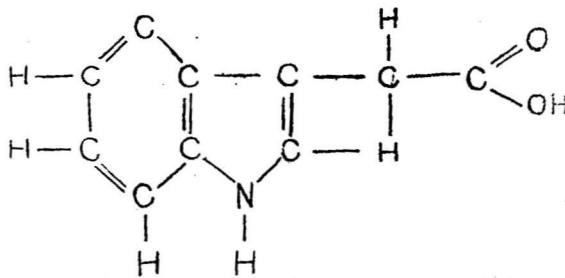
Indole 3 acetic acid (Natural Auxin)
